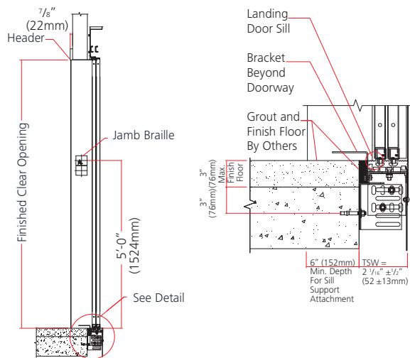
Two-speed side opening (2SSO) side jamb
