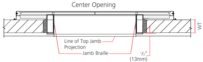
Single-speed center opening (SSCO) top jamb
