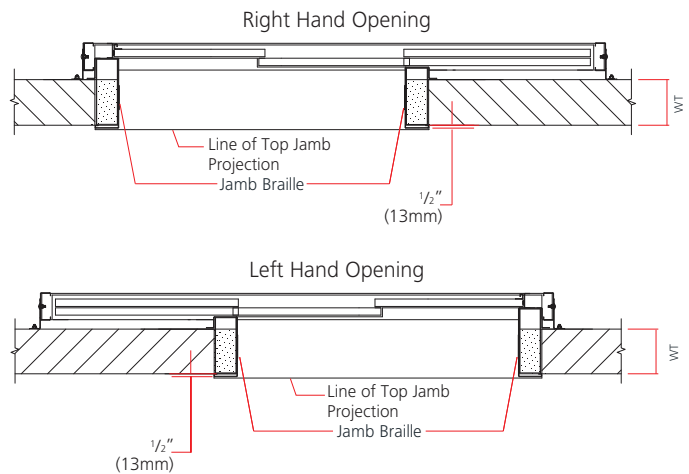
Two-speed side opening (2SSO) top jamb
