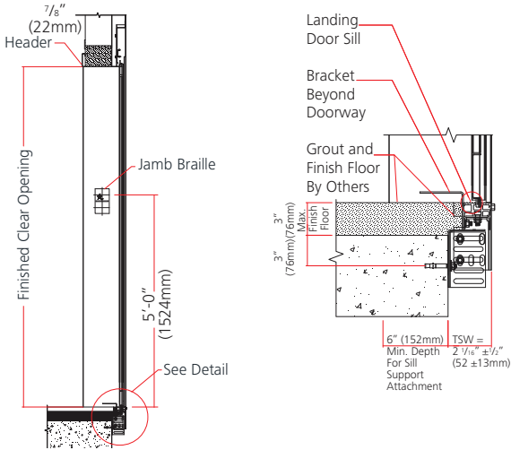
Single-speed center opening (SSCO) side jamb
