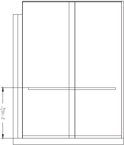
Side wall assembly 3000 lb./3500 lb.
