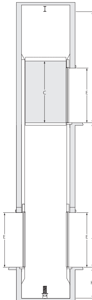
Front/rear opening
